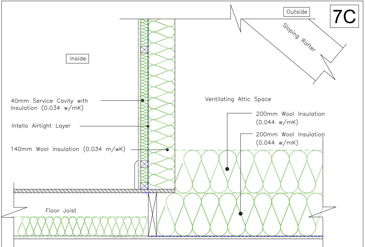
DWARF WALL (wool insulation)
