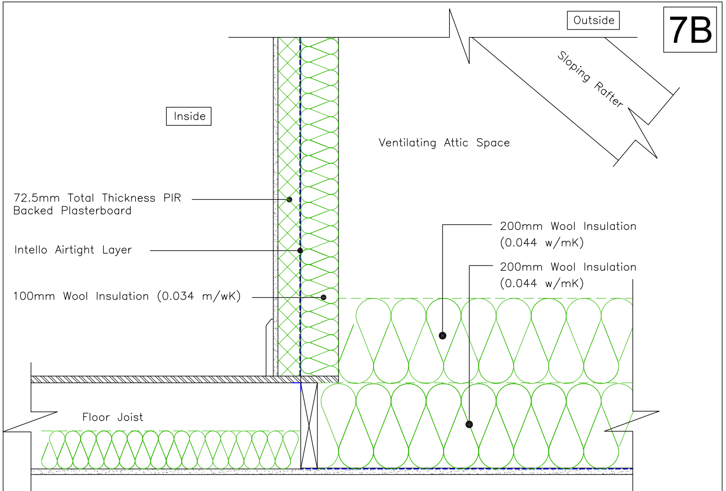
DWARF WALL (wool insulation & PIR)
