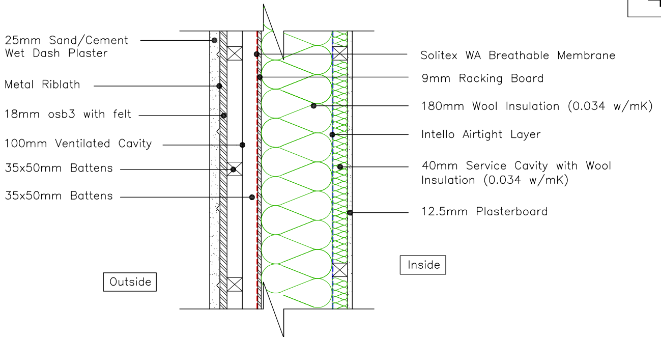
184mm DORMER CHEEK STUD WALL (wool insulation)
