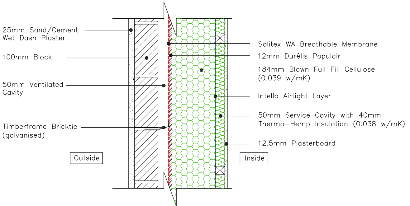
184mm TIMBERFRAME EXTERNAL WALL (cellulose & thermo-hemp insulation)
