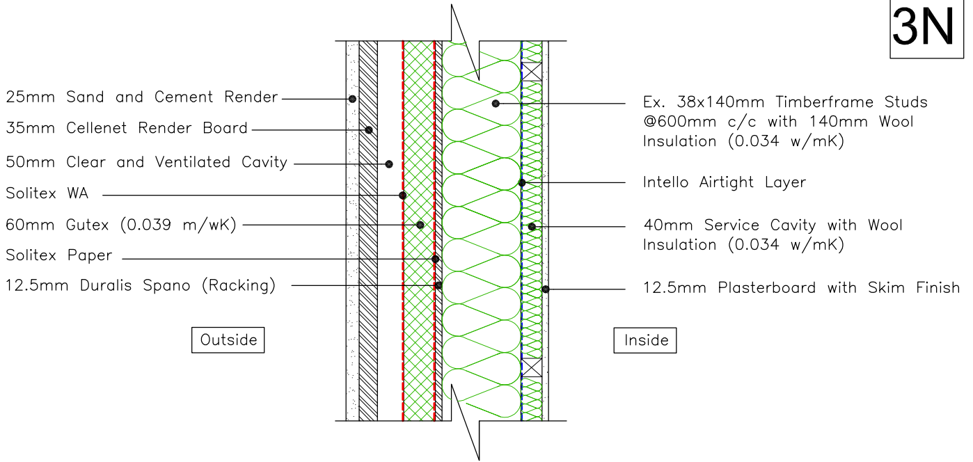
140mm Timberframe External Wall (wool insulation & gutex)
