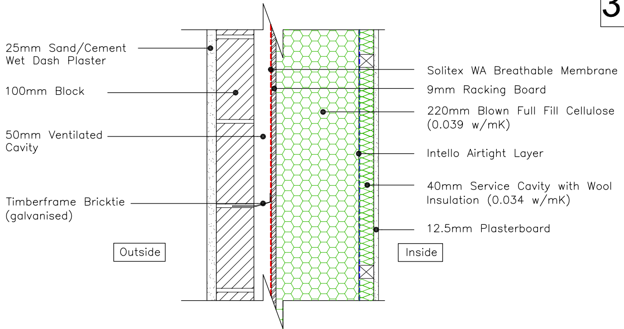
220mm TIMBERFRAME EXTERNAL WALL (cellulose & wool insulation)
