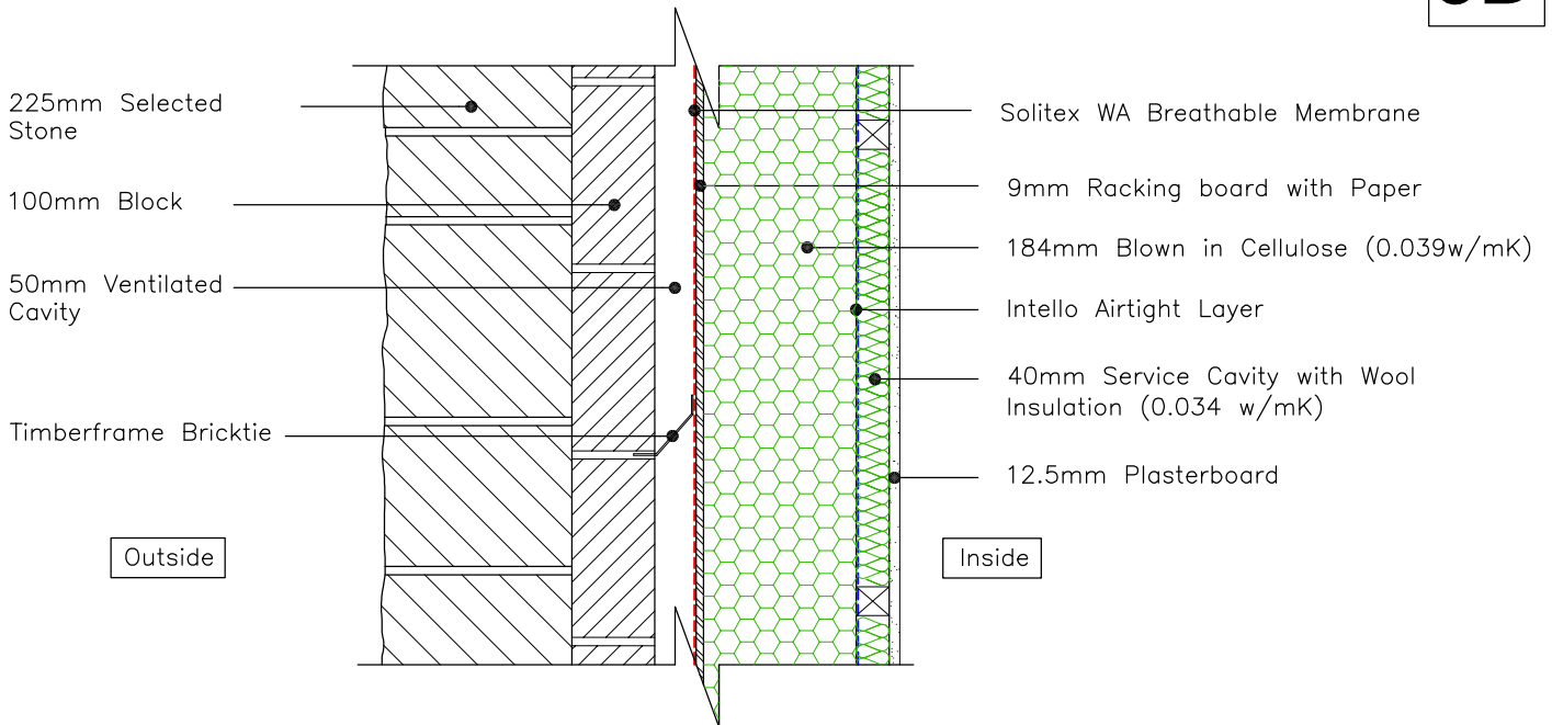
184mm TIMBERFRAME EXTERNAL WALL (cellulose)
