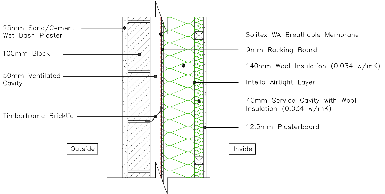
140mm TIMBERFRAME EXTERNAL WALL (wool insulation)
