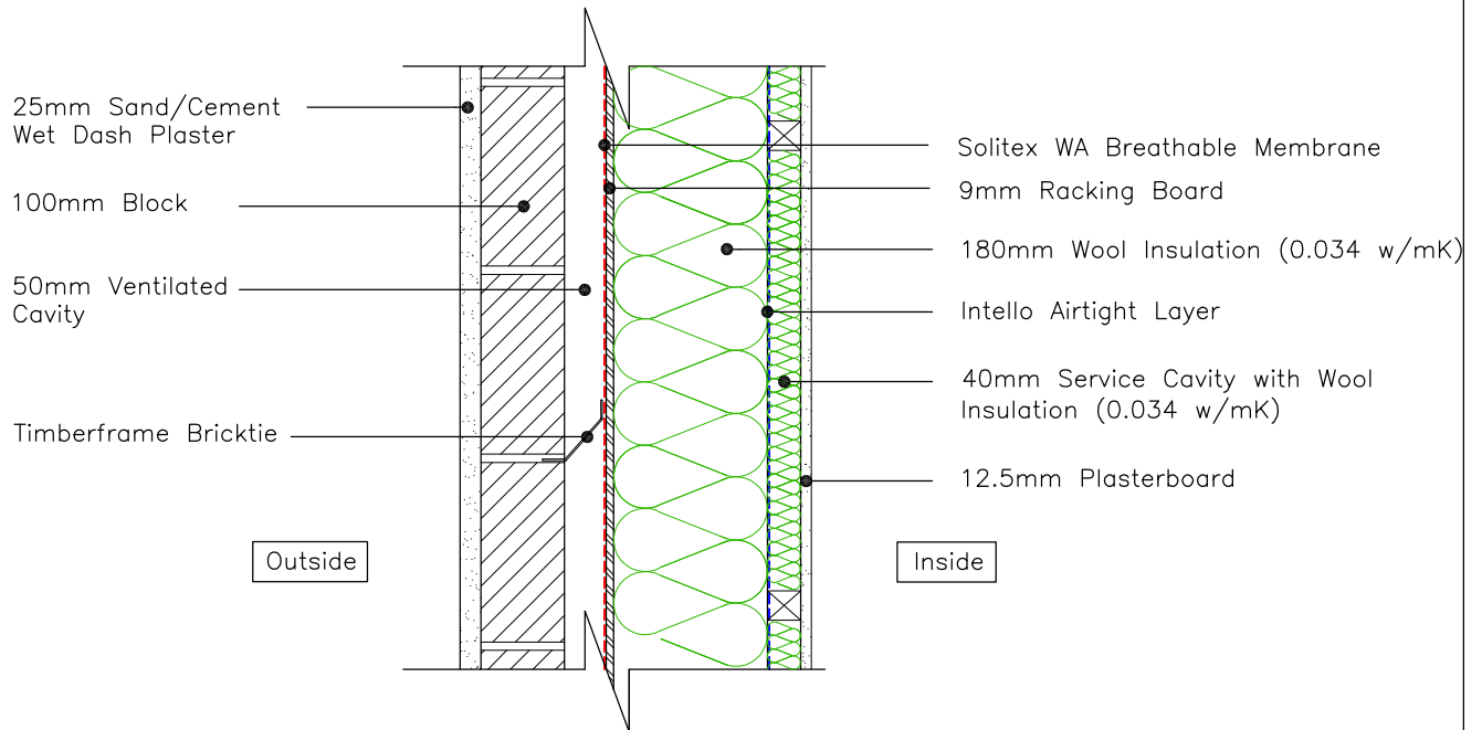
184mm TIMBERFRAME EXTERNAL WALL (wool insulation)
