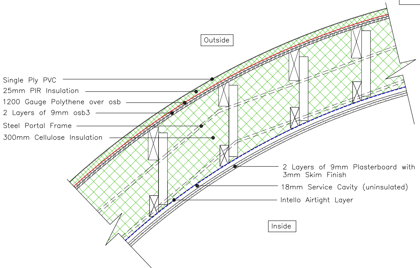
BARREL ROOF (cellulose)
