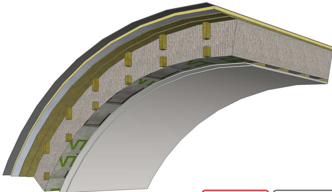
BARREL ROOF (cellulose)
