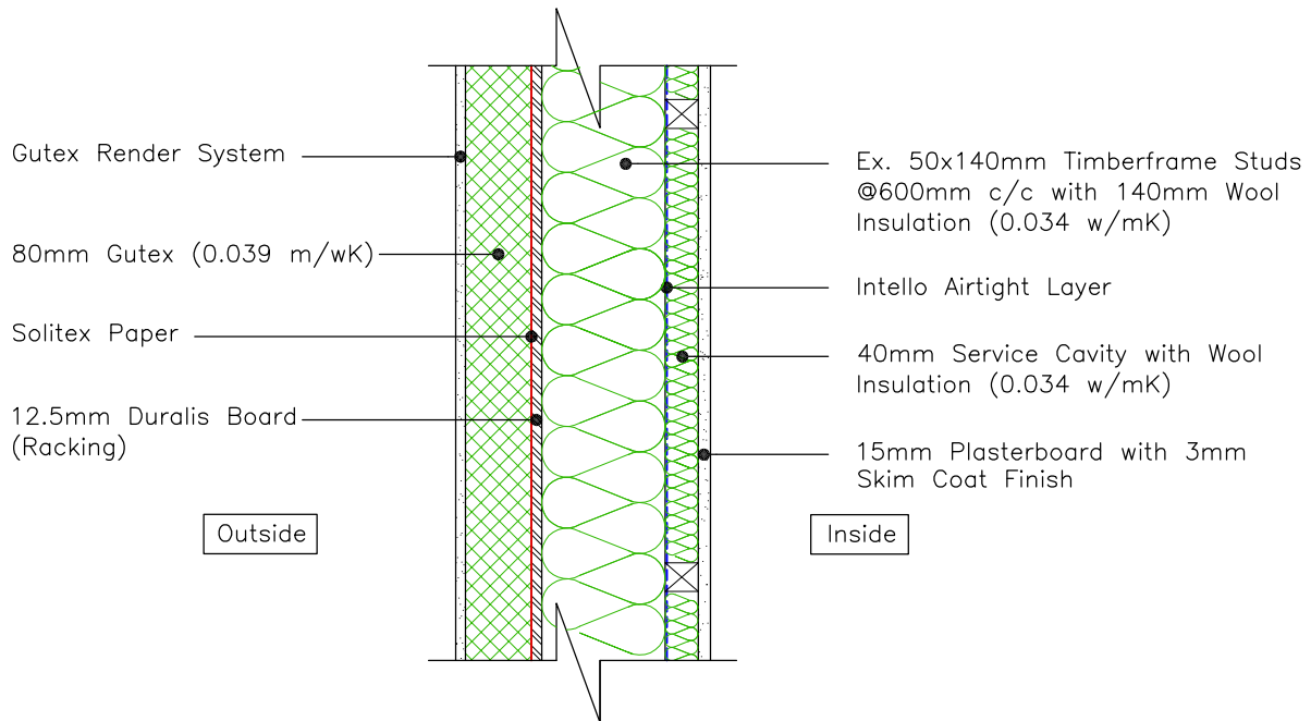
140mm DORMER CHEEK WALL (wool insulation & gutex)
