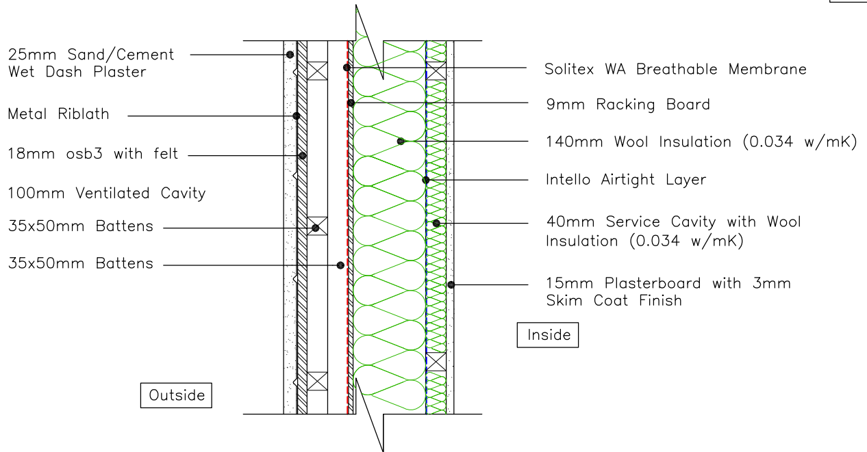
140mm DORMER CHEEK STUD WALL (wool insulation)
