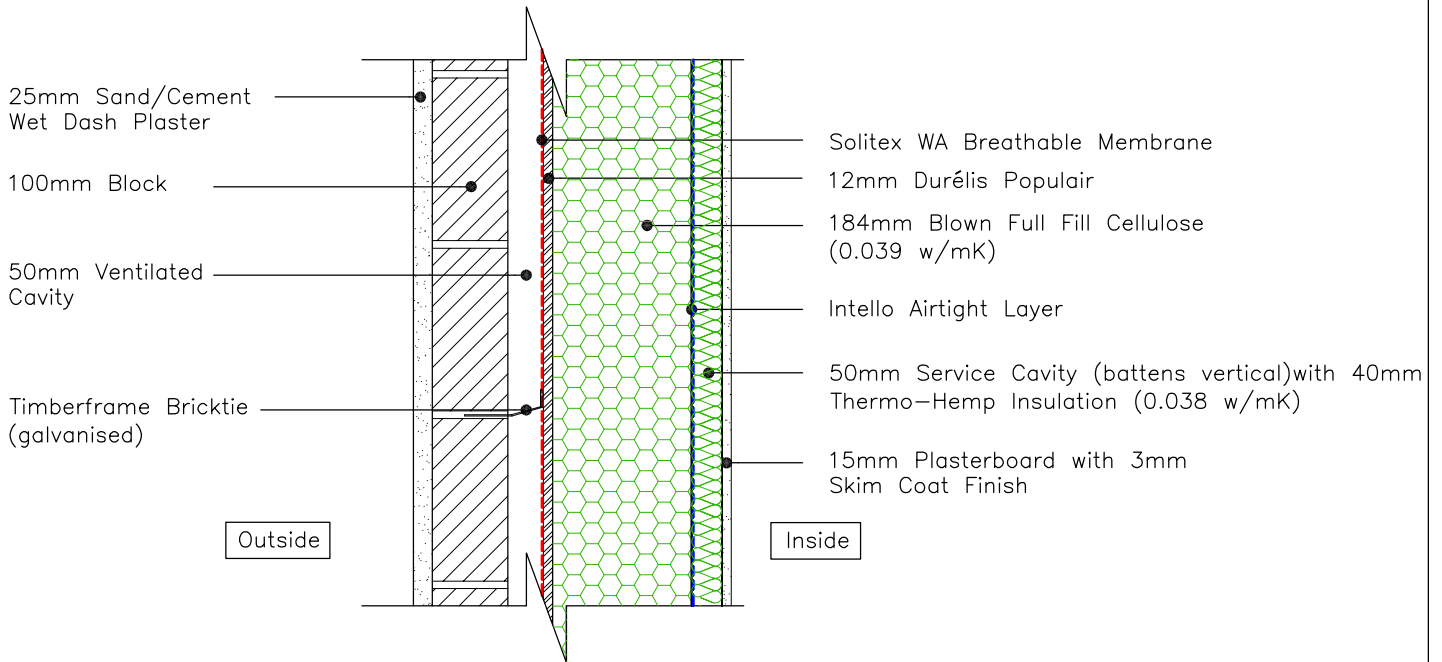
184mm TIMBERFRAME EXTERNAL WALL (cellulose & thermo-hemp insulation)
