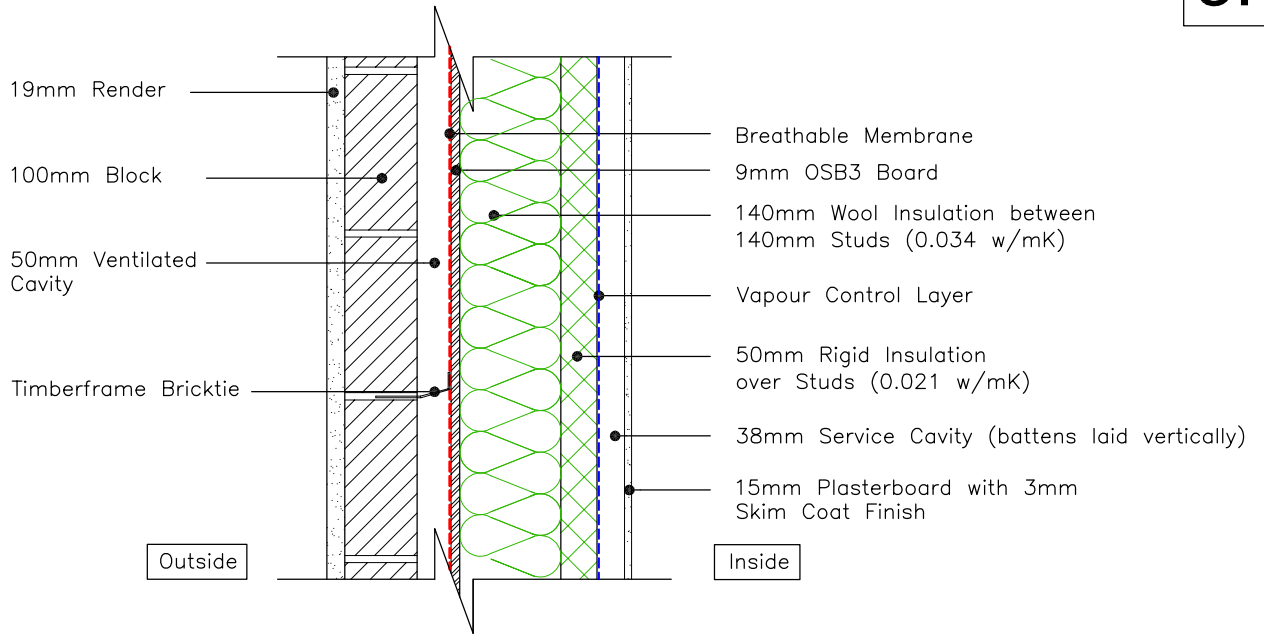
140mm TIMBERFRAME EXTERNAL WALL
