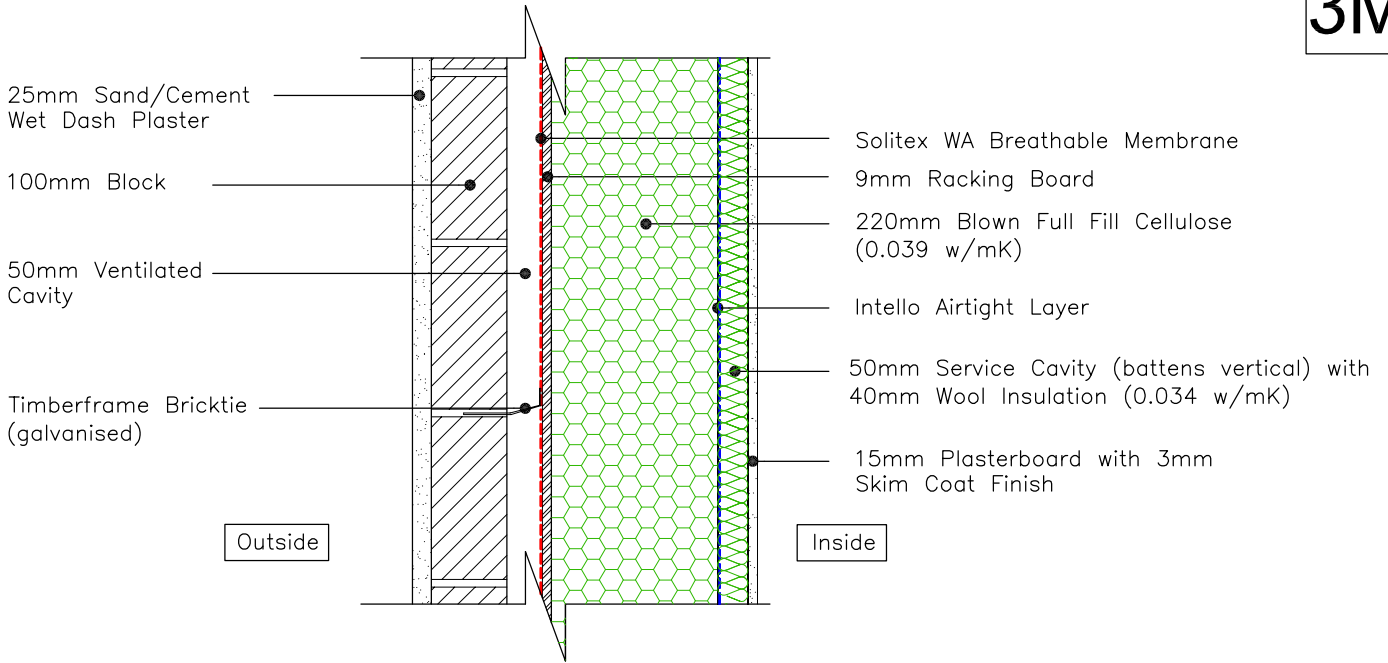
220mm TIMBERFRAME EXTERNAL WALL (cellulose & wool insulation)
