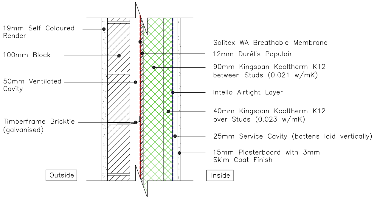
89mm TIMBERFRAME EXTERNAL WALL
