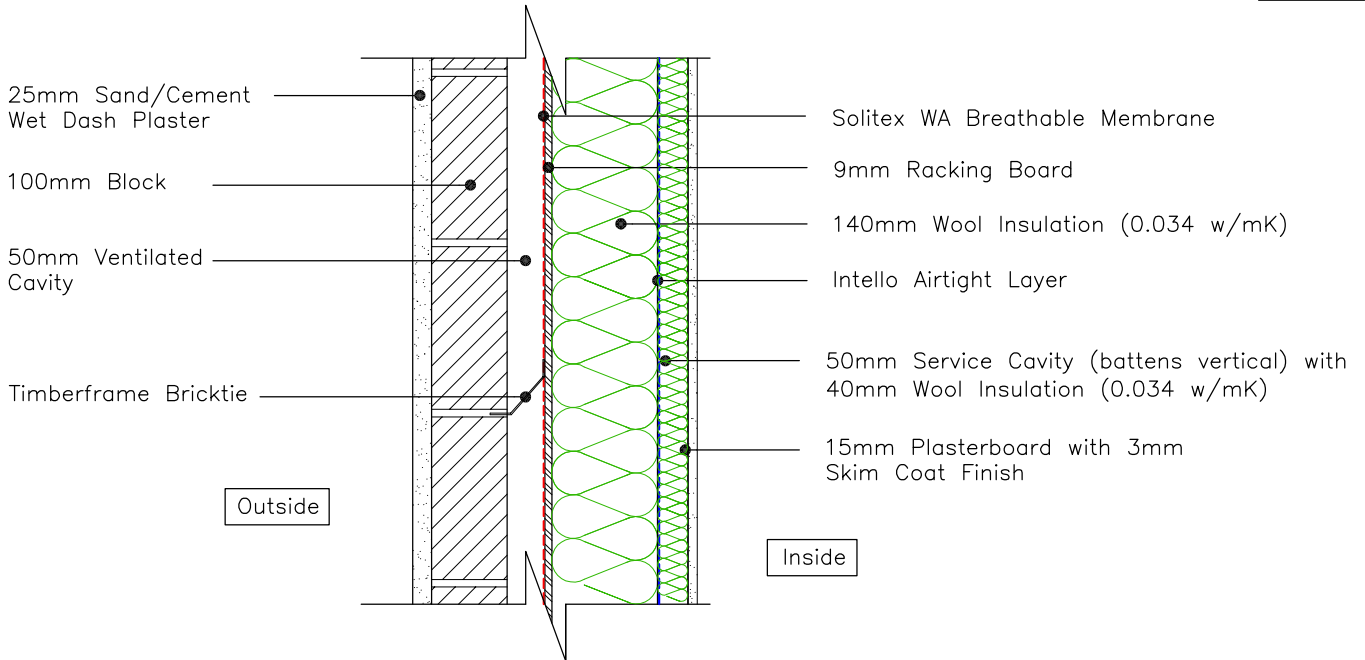
140mm TIMBERFRAME EXTERNAL WALL (wool insulation)
