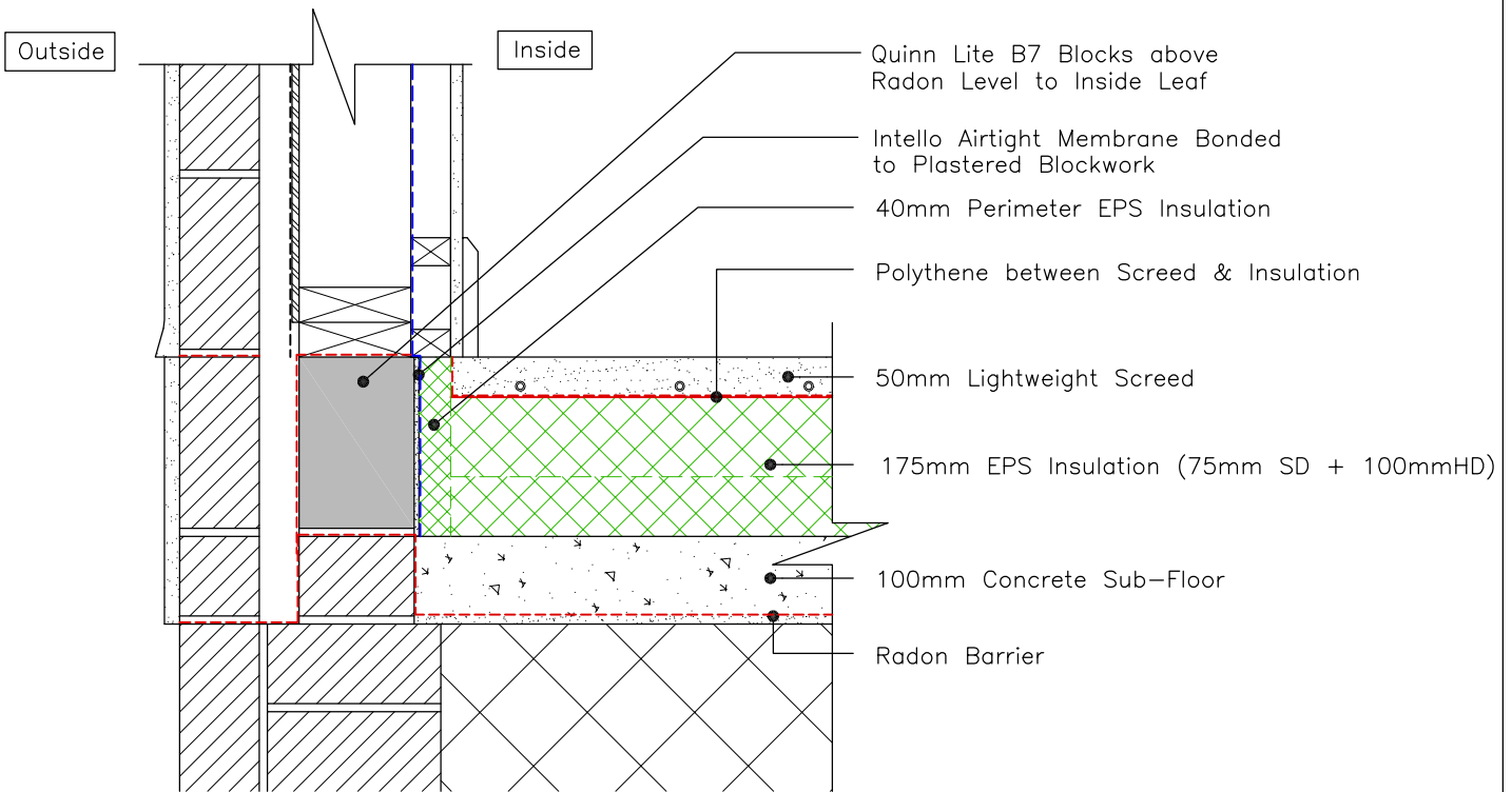
GROUND FLOOR - 140mm External Stud
