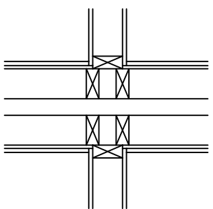
DETAIL A HORIZONTAL SECTION AT PARTY WALL & INTERNAL PARTITION JUNCTION.
