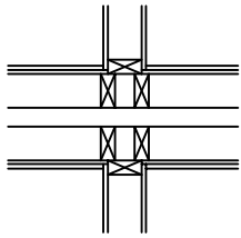
DETAIL A SECTIONAL SECTION AT PARTY WALL & INTERNAL PARTITION JUNCTION.
